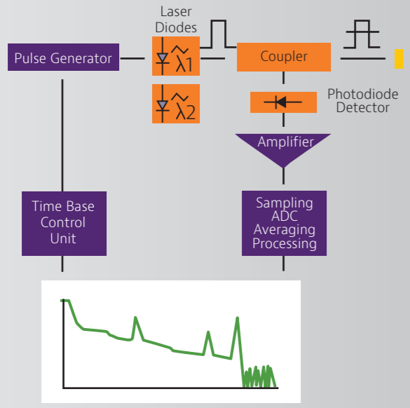
A schematic diagram showing OTDR technology
